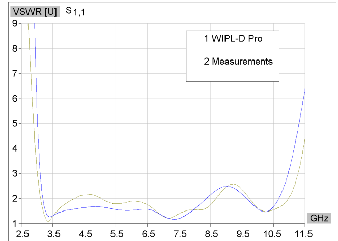
VSWR overlay in range 2.5-11.5 GHz
