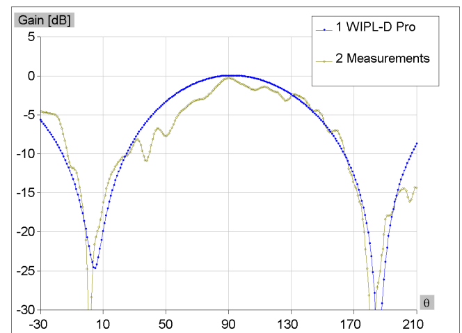
|E| [dB] in E plane 4 GHz
