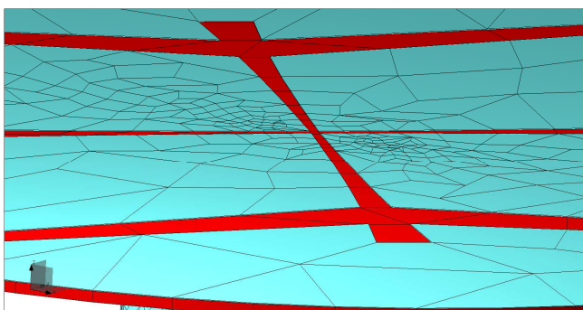
Upper side of substrate mesh (zoom in)
